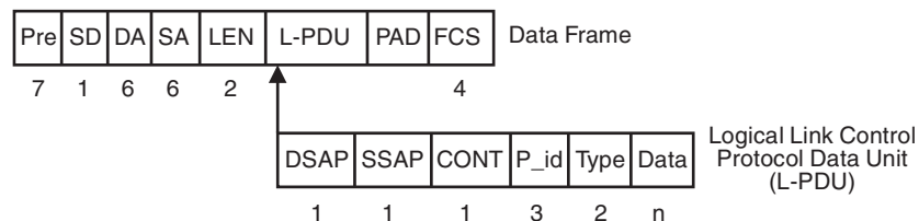
Figure 112. Format of an IEEE 802.3 frame
