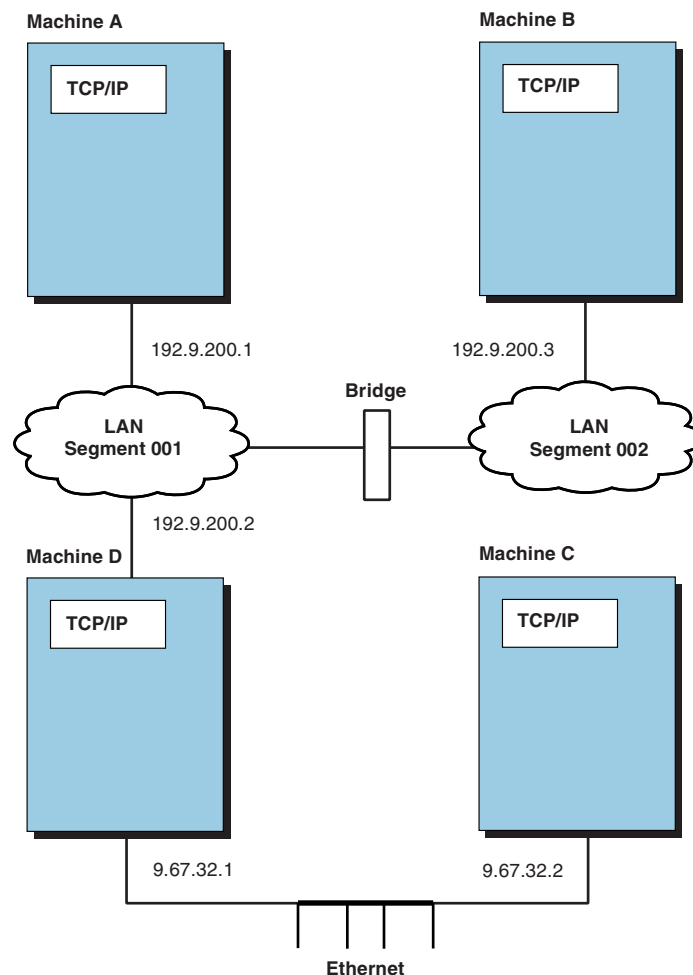
Figure 117. Routing and bridging
