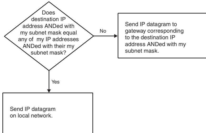
Figure 120. Routing algorithm with subnets
