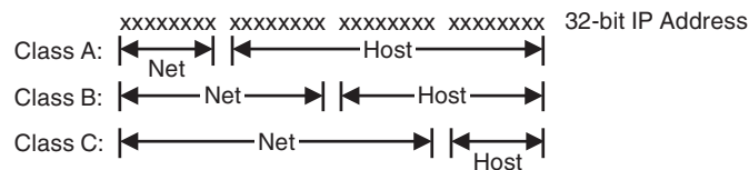
Figure 115. Classes of IPv4 addresses
